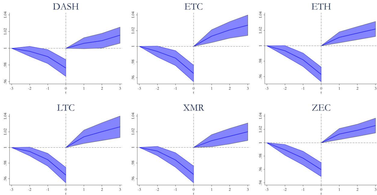
Figure 7. Prices of Bitcoin and Other Cryptocurrencies around High-Flow Events. Panel A shows Bitcoin prices in 3 hours before and after the 87 high-flow hours. Prices are scaled to one at time -3 before the event and at time zero after the event. Scaled prices are averaged across the events. These 87 events are defined as hours with at least 200 Bitcoin-denominated Tether flow from Bitfinex to Poloniex and Bittrex and at least 200 inflow of Bitcoins back to Bitfinex in the prior hour, conditional on Tether issuance in the prior three days and negative returns in the prior hour. Panel B shows similar results for other major cryptocurrencies.
